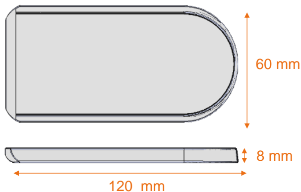
Dimensions coque
